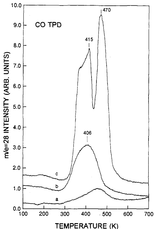
Figure 8. CO TPD spectra obtained following CO saturation exposure: (a) CO TPD spectrum acquired after a Ru(0001) surface is saturated with the methylidyne species; (b) CO TPD obtained from the surface corresponding to the upper spectrum of Figure 3; and (c) CO TPD spectrum of a clean Ru(0001) surface.
