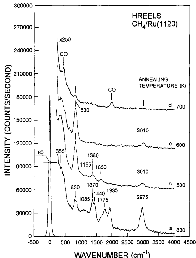
Figure 6. HREELS spectra acquired after methane activation over a Ru(11 \bar{2} 0) surface as a function of the UHV annealing temperature. The reaction of methane with a Ru(11 \bar{2} 0) catalyst was carried out at the reaction temperature of 330 K with 5 Torr CH 4 for 120 s. The spectra were collected at E_p \approx 2.2 eV and at the specularly reflected beam direction.
