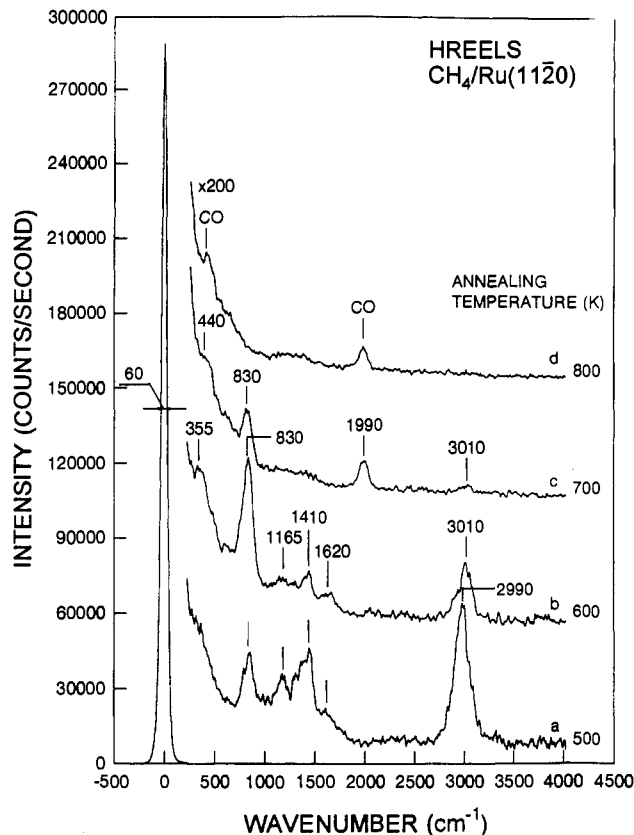
Figure 7. HREELS spectra acquired following methane decomposition on a Ru(11 \bar{2} 0) surface versus the UHV annealing temperature. The reaction of methane with a Ru(11 \bar{2} 0) catalyst was carried out at the reaction temperature of 500 K with 5 Torr CH 4 for 120 s. The spectra were collected at E_p \approx 2.2 eV and at the specularly reflected beam direction.
